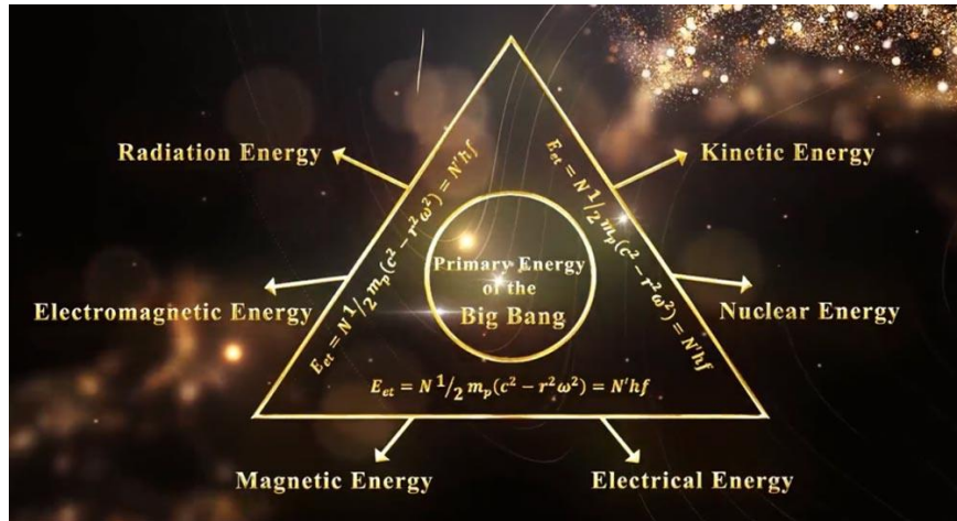
Figure 1. Saleh Comprehensive Equation of Theory of Everything
